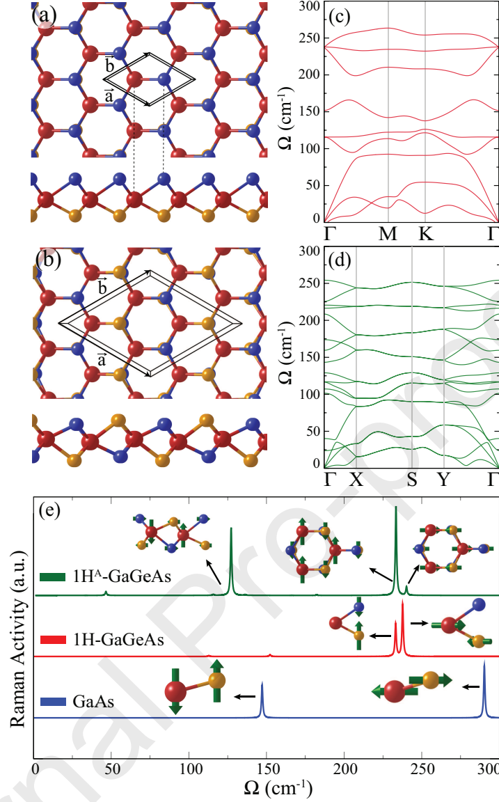
FIG. 3: The top and side views of single-layer (a) 1H-GaGeAs and (b) 1H A -GaGeAs. (c) and (d) The corresponding phonon band dispersions, respectively. (e) Raman spectrum of each GaGeAs structures and that of single-layer GaAs for comparison. The vibrational characteristics of some prominent Raman active modes are shown in the inset.
