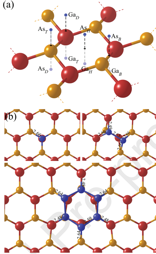
FIG. 1: (a) Possible adsorption sites for Ge atom on each atomic plane of single-layer GaAs. (b) Illustration of the growth of hexagonal Ge_N clusters ( N=2,6 ) starting from the single Ge adsorption on favorable Ga_D site. The atomic bond lengths are given on each corresponding bond. Blue, red, and orange colors represent Ge, Ga and As atoms, respectively.
